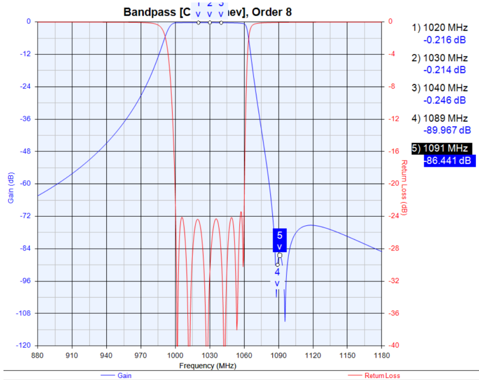
Insertion loss , Return loss ,Rejection
