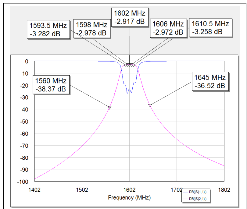
[ SIMULATION CURVE ]
