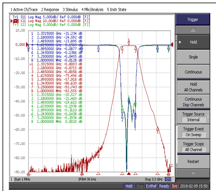
[ TEST CURVE ]
