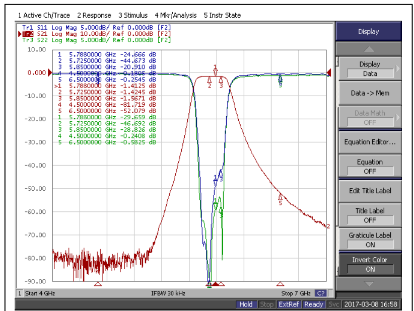
[ TEST CURVE ]
