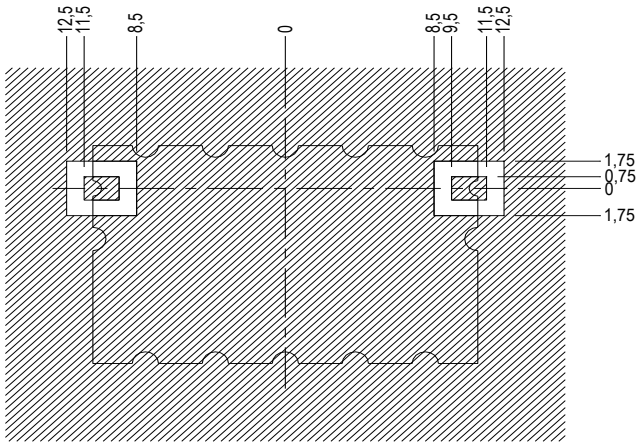
LAND PATTERN
