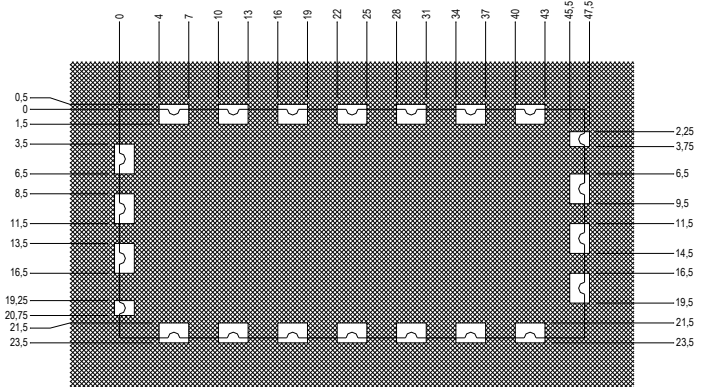
[ SOLDER RESISTOR ]
