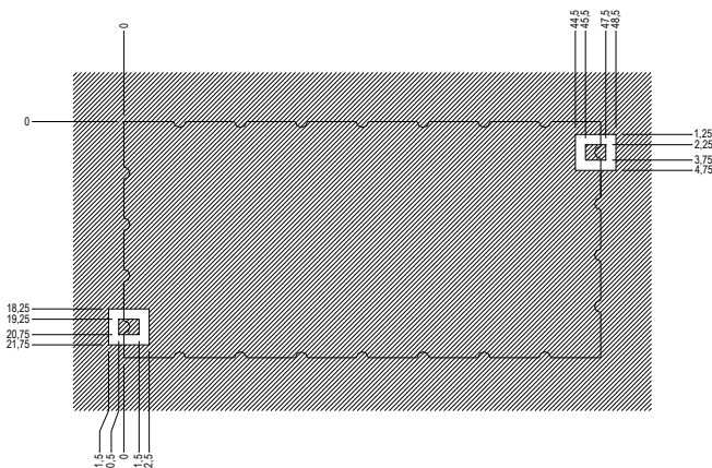
[ LAND PATTERN ]
