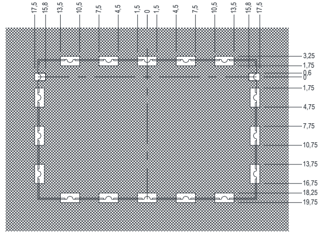
SOLDER RESISTER
