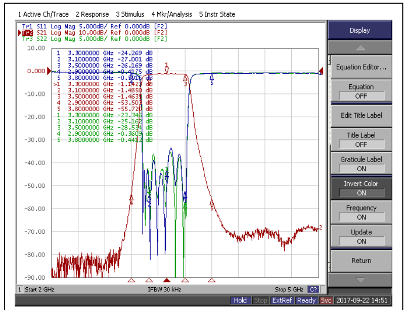
[ SIMULATION CURVE ]
