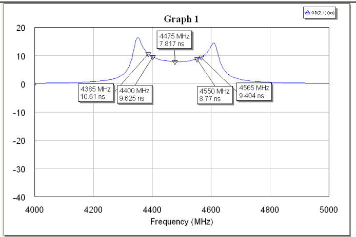
Group Delay
