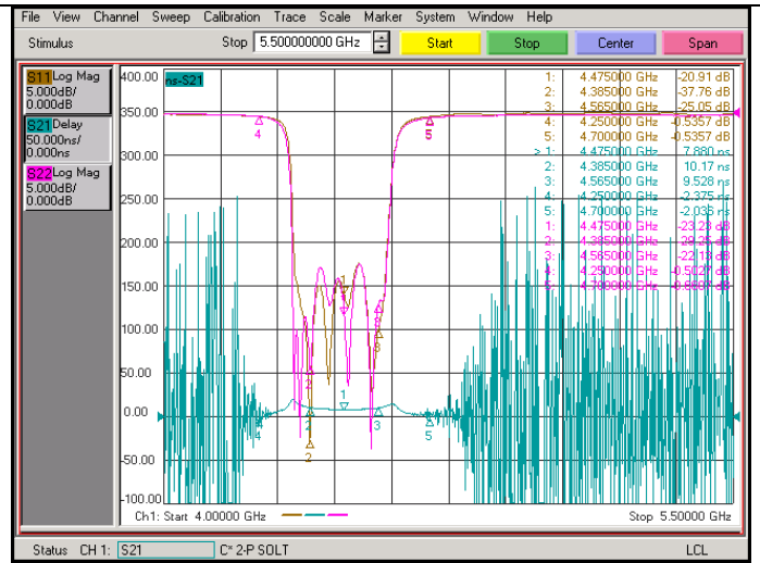
Group Delay
