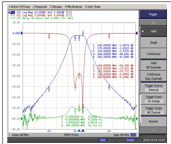
[ TEST CURVE ]
