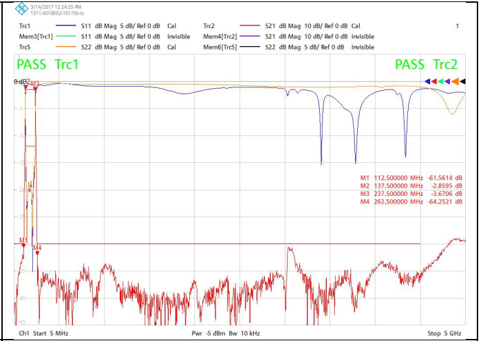
Harmonics
