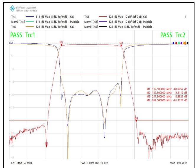
[ TEST CURVE ]
