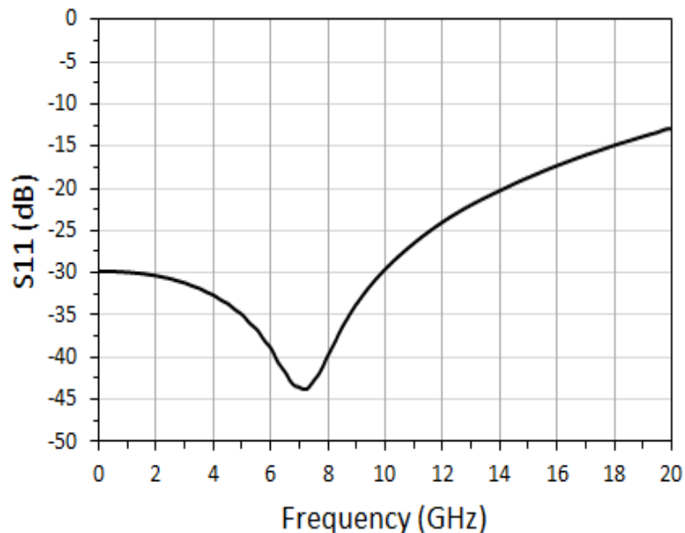
Return Loss vs, Frequency
