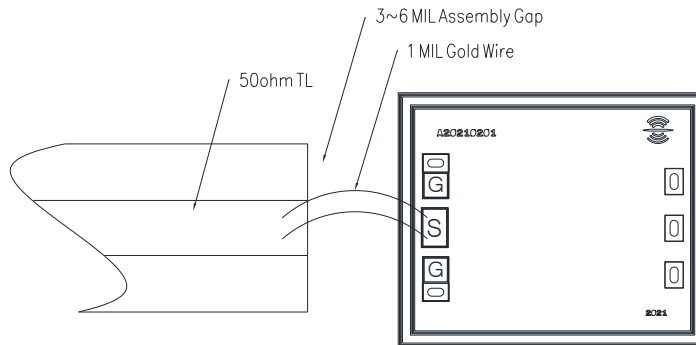
Assembly Diagram
