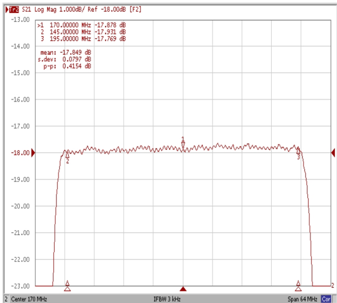
Ripple Variation F_o \pm 25\text{MHz}
