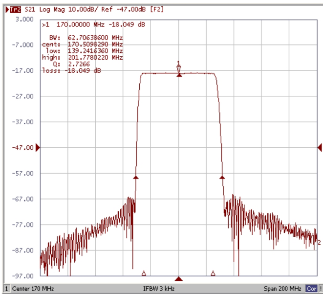
-40dB Bandwidth
