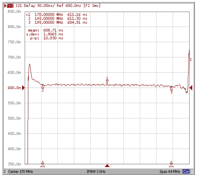
Group Delay Variation F_o \pm 25\text{MHz}
