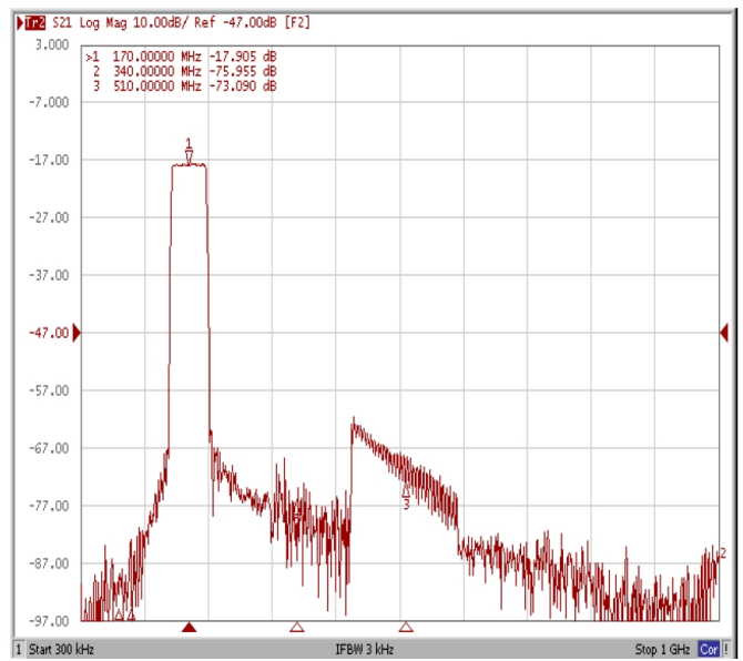
Harmonics
