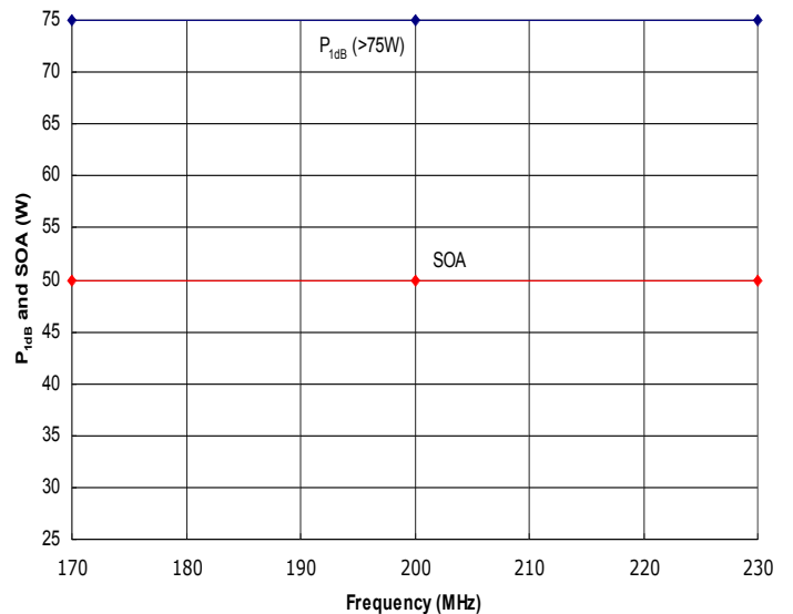
Figure 4: HD31369 Typical P 1dB and Safe Operating Area (SOA). The amplifier is capable of delivering much more power than it is safe to generate. Do not exceed the SOA shown above without first contacting HD Communications Corp. to discuss your application.
