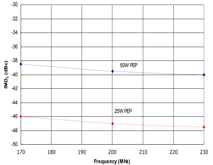
Figure 2: HD31369 Typical IMD 3 @ 50W and 25W PEP, Δf=10kHz and Δf=100kHz.
