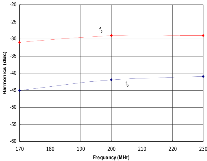
Figure 3: HD31369 Typical f 2 and f 3 @ P out =50W.
