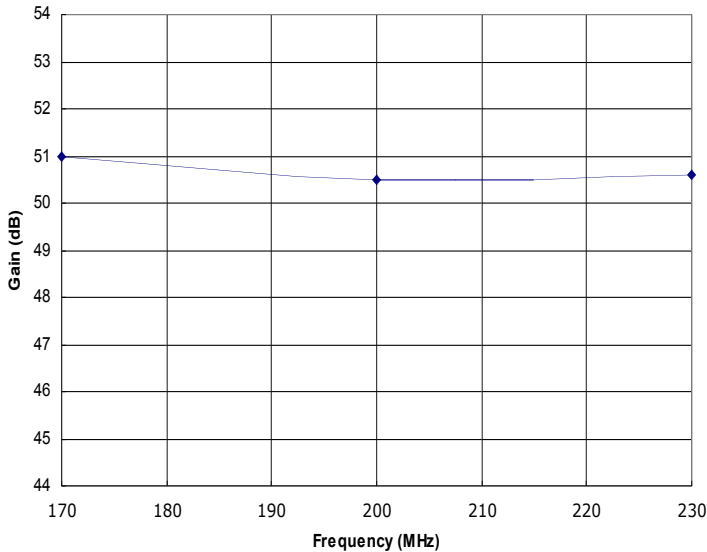
Figure 1: HD31369 Typical Gain @ P out =50W.
